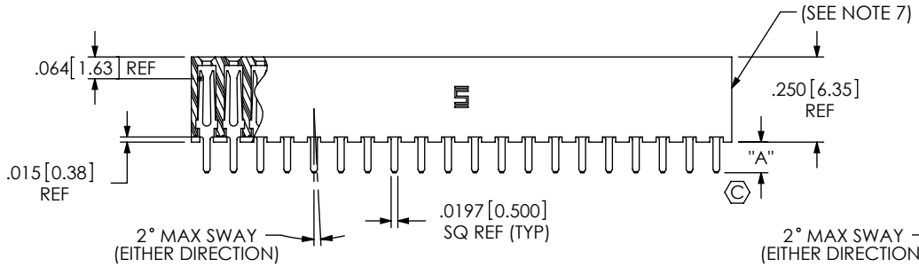
FIG 1 SQT-120-01-XX-6 SHOWN
