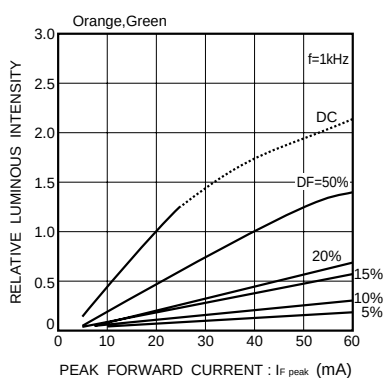
Fig. 21 Luminous intensity vs. peak forward current
