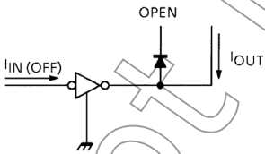
4. I_{IN(OFF)}
