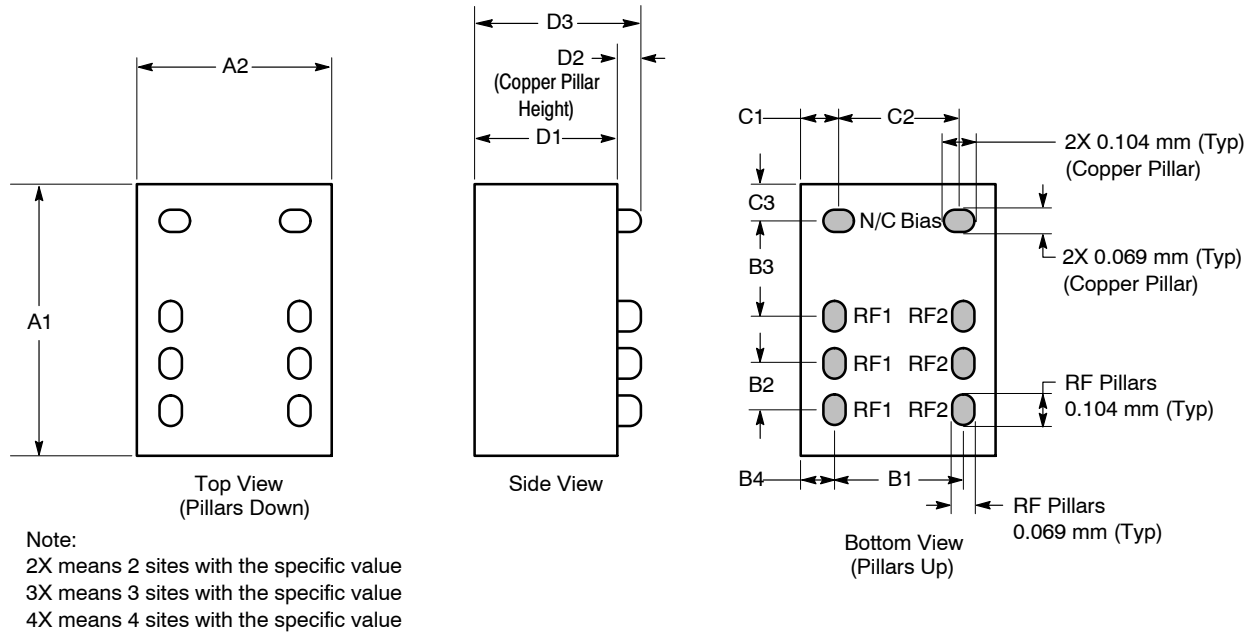
Figure 7. WLCSP Package Dimensions
