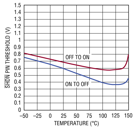
SHDN Pin Thresholds
