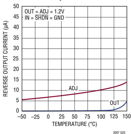
Reverse-Output Current
