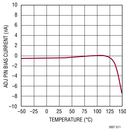
ADJ Pin Bias Current
