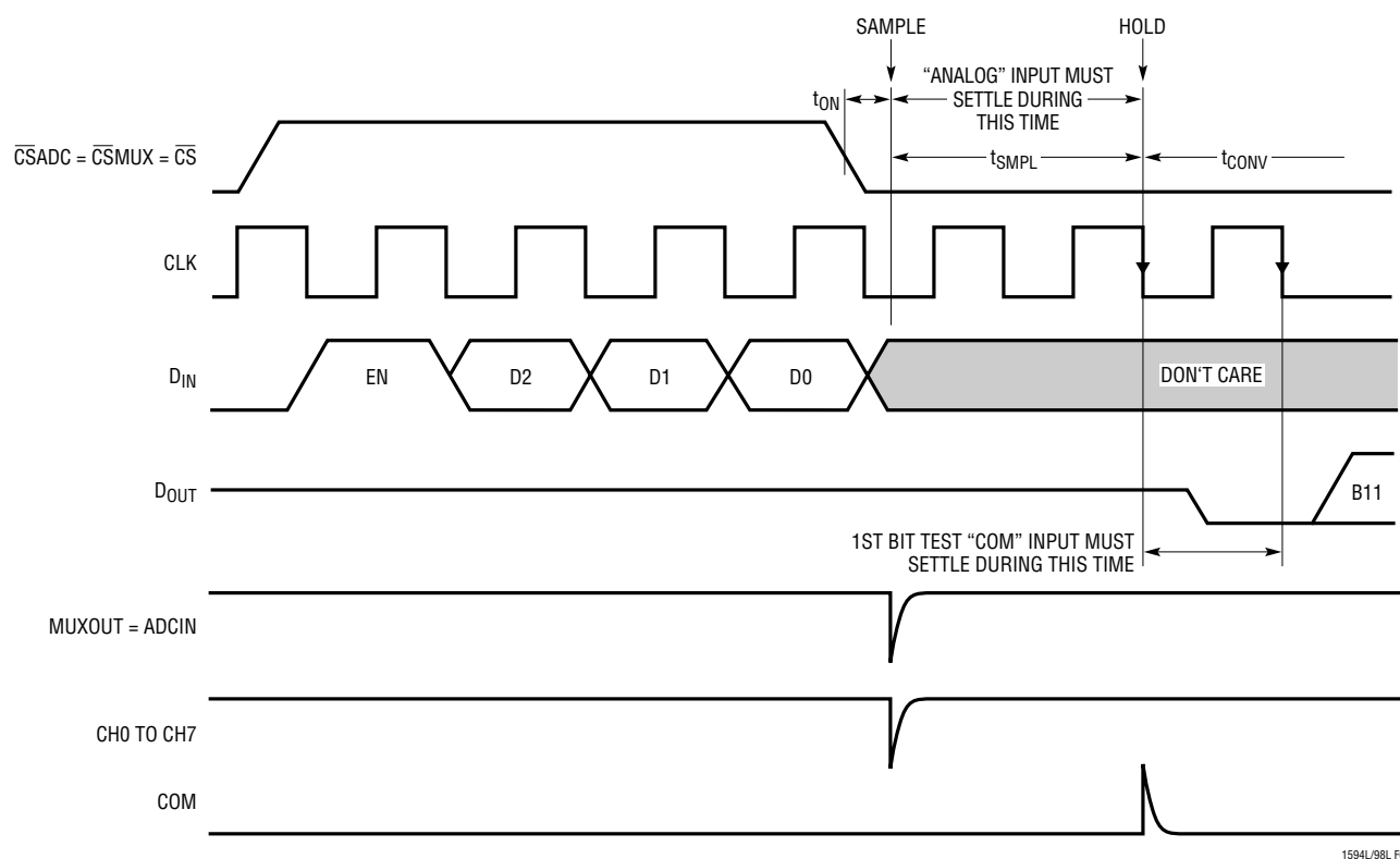
Figure 7. LTC1594L/LTC1598L ADCIN and COM Input Settling Windows
