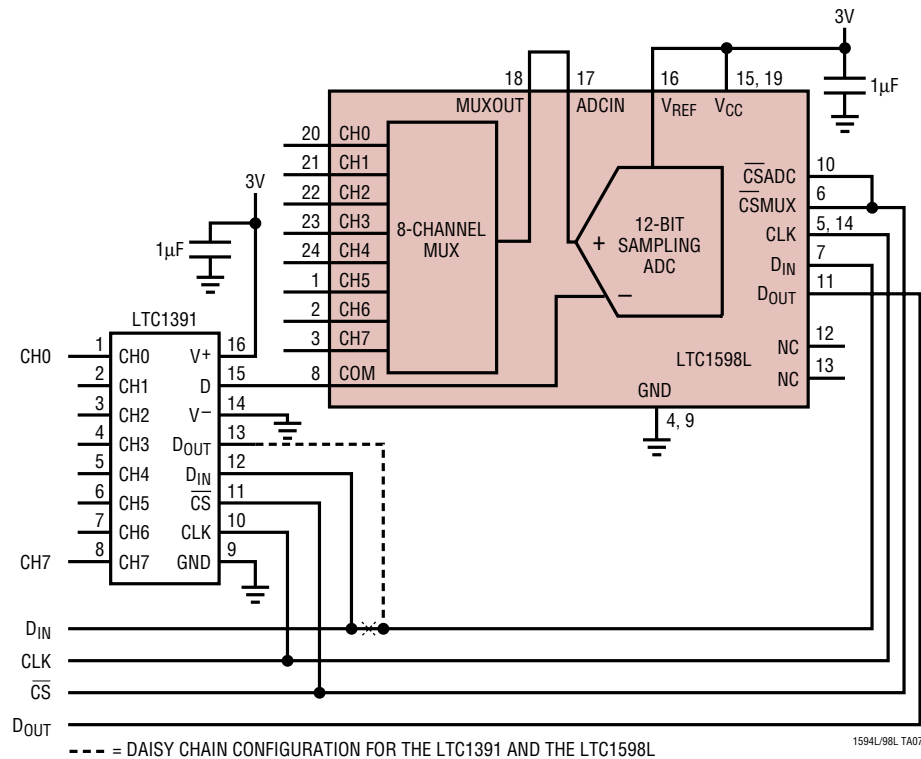
Using the LTC1598L and LTC1391 as an 8-Channel Differential 12-Bit ADC System
