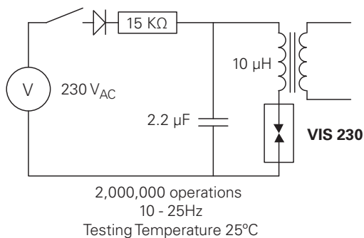
VIS 230 Life Test Circuit
