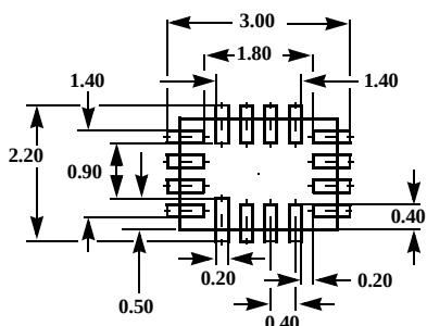
10 LAND PATTERN
