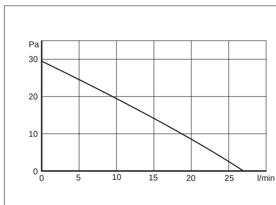
AIR PERFORMANCE DIAGRAM
