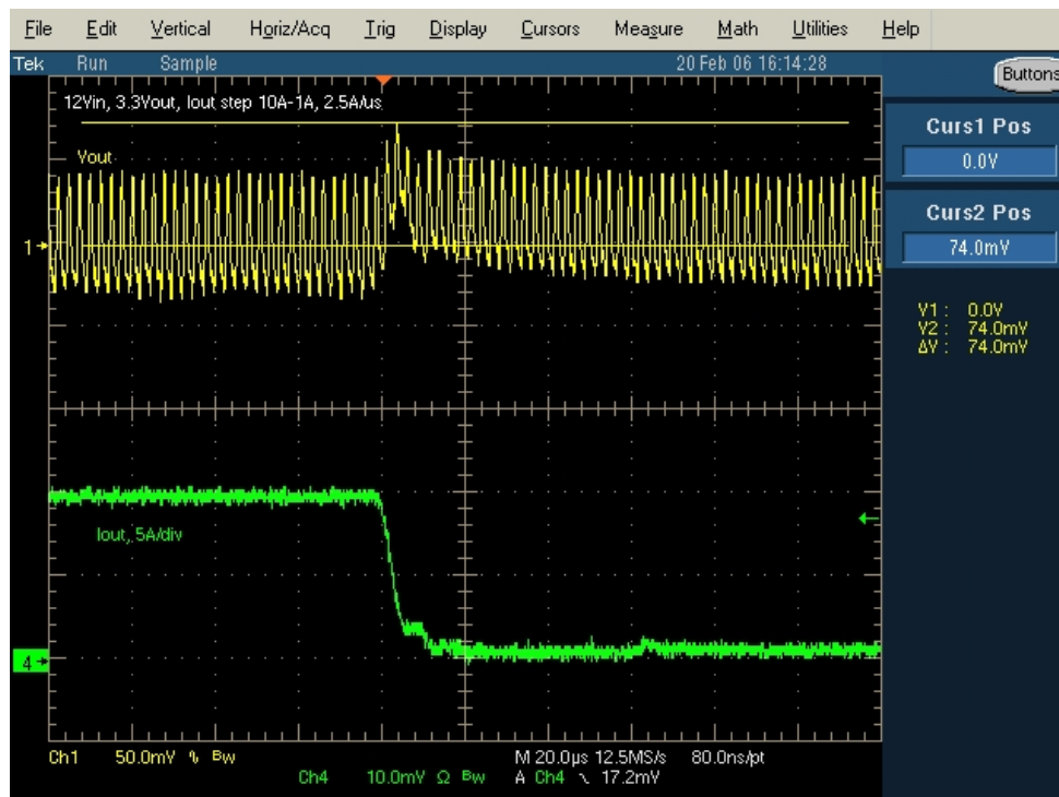
Figure 10: Output Voltage overshoot due to 10A to 1A load step, di/dt=2.5A/\mu s
