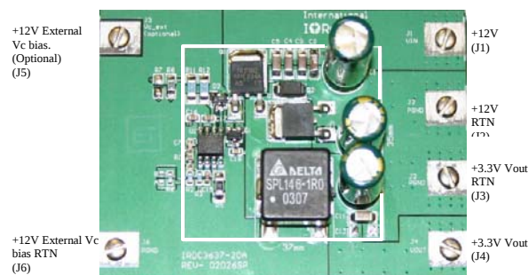
Figure 1: IRPP3637-18A Electrical Connection Diagram
