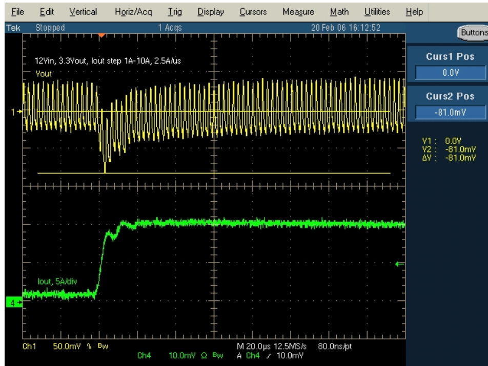
Figure 9: Output Voltage undershoot due to 1A to 10A load step, di/dt=2.5A/\mu s
