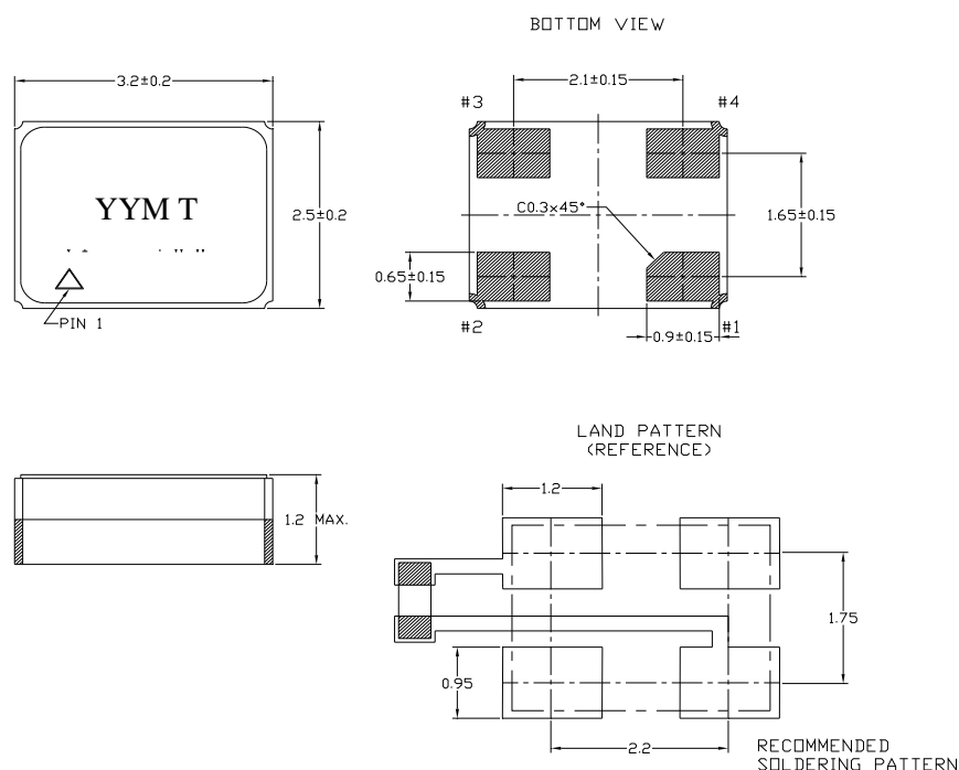
Figure 7, Package drawing
