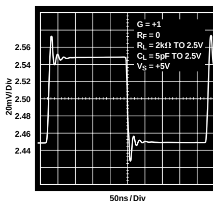
Figure 36. 100 mV Step Response
