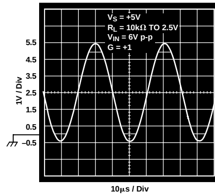
Figure 31. Output Voltage
