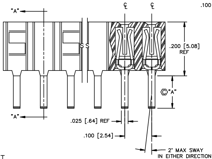
SECT. "B-B"
