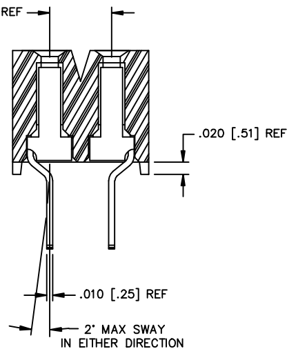
SECT. "A-A"
