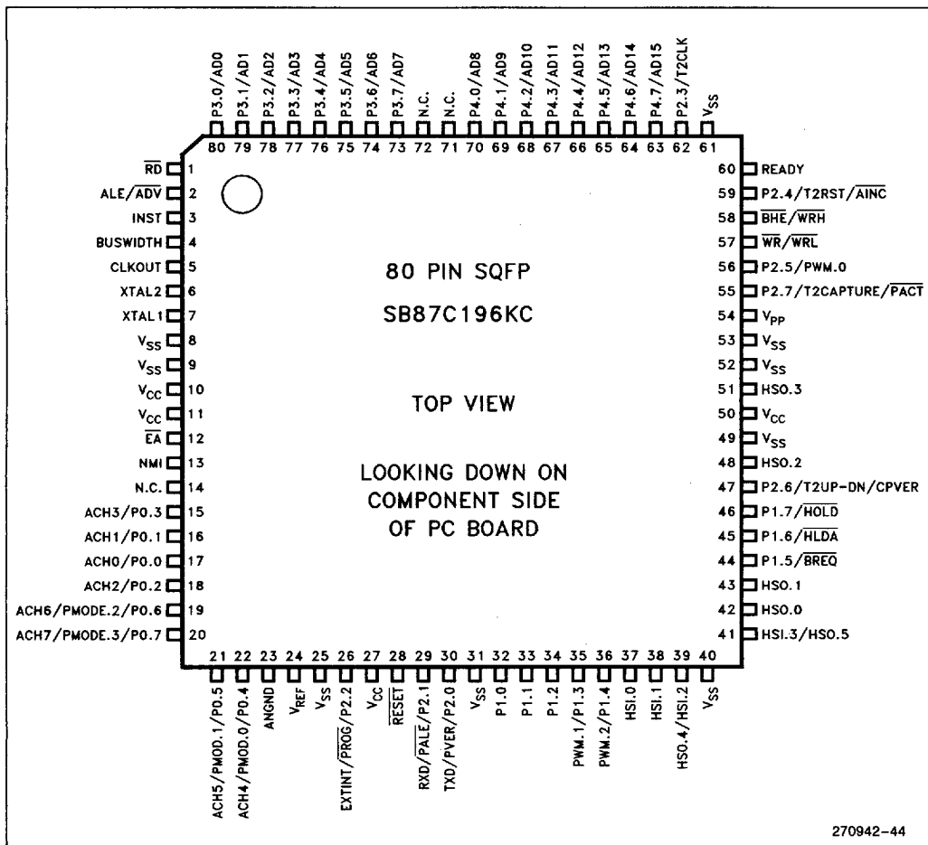
Figure 6. 80-Pin SQFP Package
