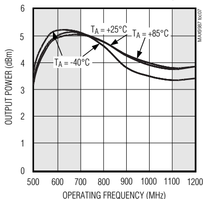
OUTPUT POWER vs. FREQUENCY, PLL
