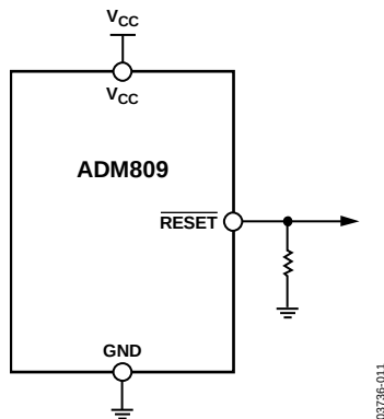
Figure 12. Ensuring a Valid Reset Output Down to V_{CC} = 0 V
