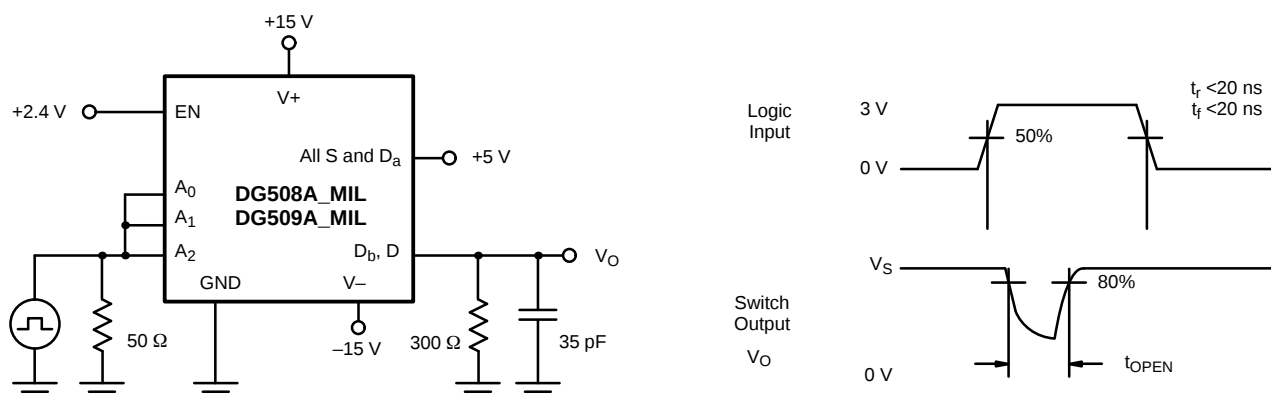
FIGURE 4. Break-Before-Make Interval
