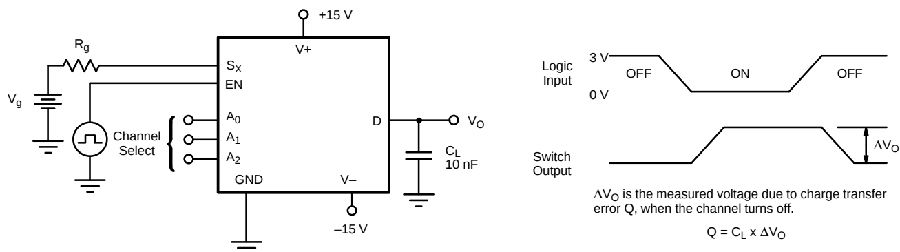
FIGURE 5. Charge Injection
