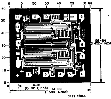
CD4001UB
