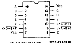
CD4025UB
