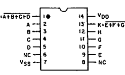
CD4002UB
