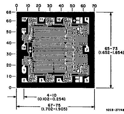
CD4002UB
