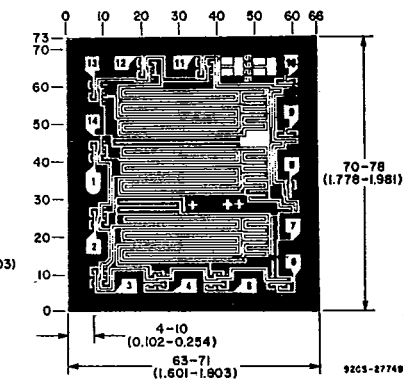
CD4025UB
