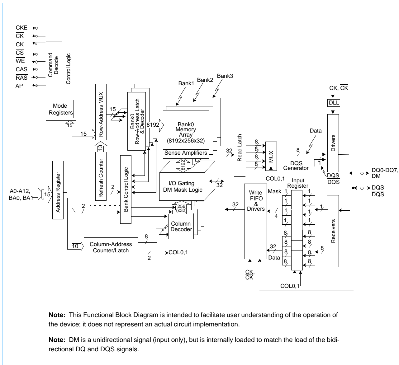
Block Diagram 8Mbit x 8 I/O x 4 Internal Memory Banks
