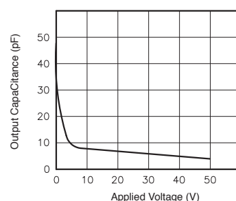
Fig.12 Applied voltage vs. output capacitance Across terminals 3 and 4 pin Frequency: 1MHz Ambient temperature: 25°C
