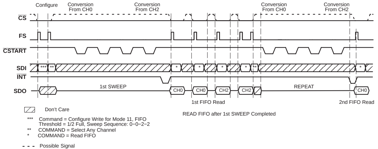
Figure 19. Mode 11, \overline{\text{CSTART}} Triggers Samplings/Conversions, FS Initiates SELECT Operation
