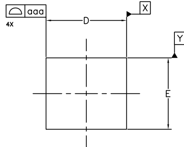
Figure 21. 50-Ball WFBGA Mechanical Drawing
