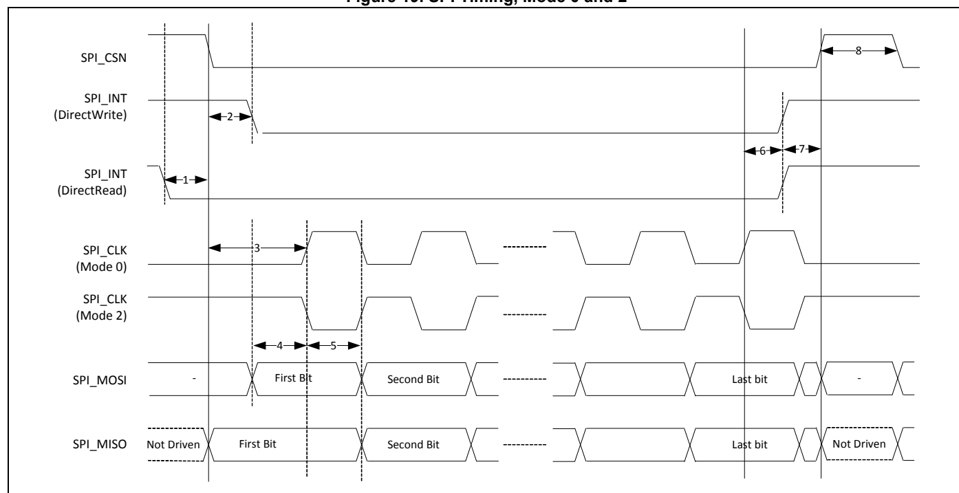
Figure 19. SPI Timing, Mode 0 and 2
