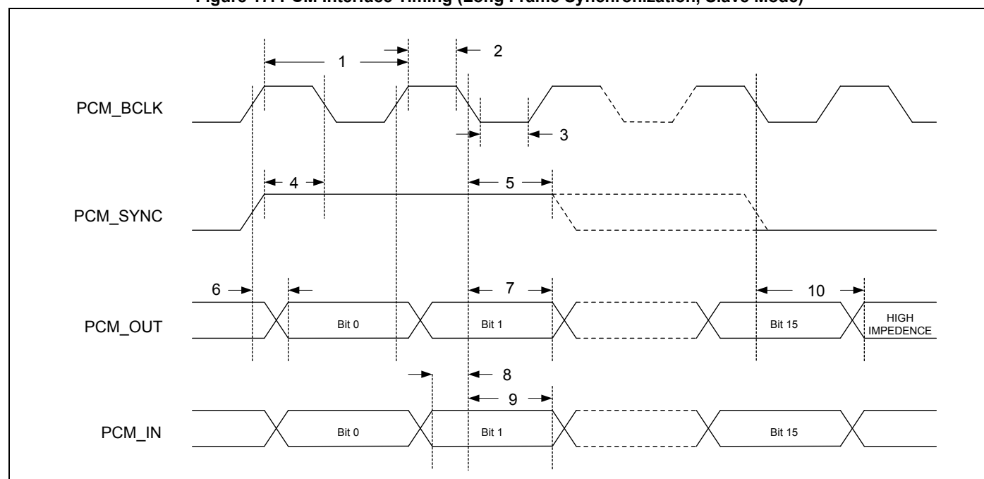
Figure 17. PCM Interface Timing (Long Frame Synchronization, Slave Mode)
