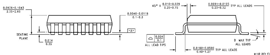
-B- 0.5977-0.4133 10.10-10.50 16 15 14 13 12 11 10 9 LEAD NO. 1 IDENTIFICATION 0.2914-0.2992 7.4-7.6 0.3940-0.4190 10.00-10.65 -C- 1 2 3 4 5 6 7 8 0.050 1.27 0.0138-0.0200 0.350-0.508 TYP 0.010 0.25 M A C S B
