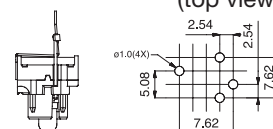
PCB layout (top view)
