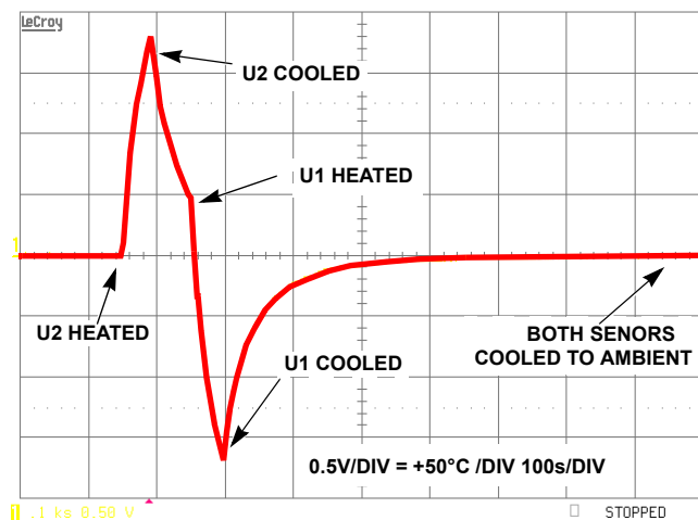
FIGURE 10. ISL71590SEH DIFFERENTIAL CONFIGURATION OPERATION
