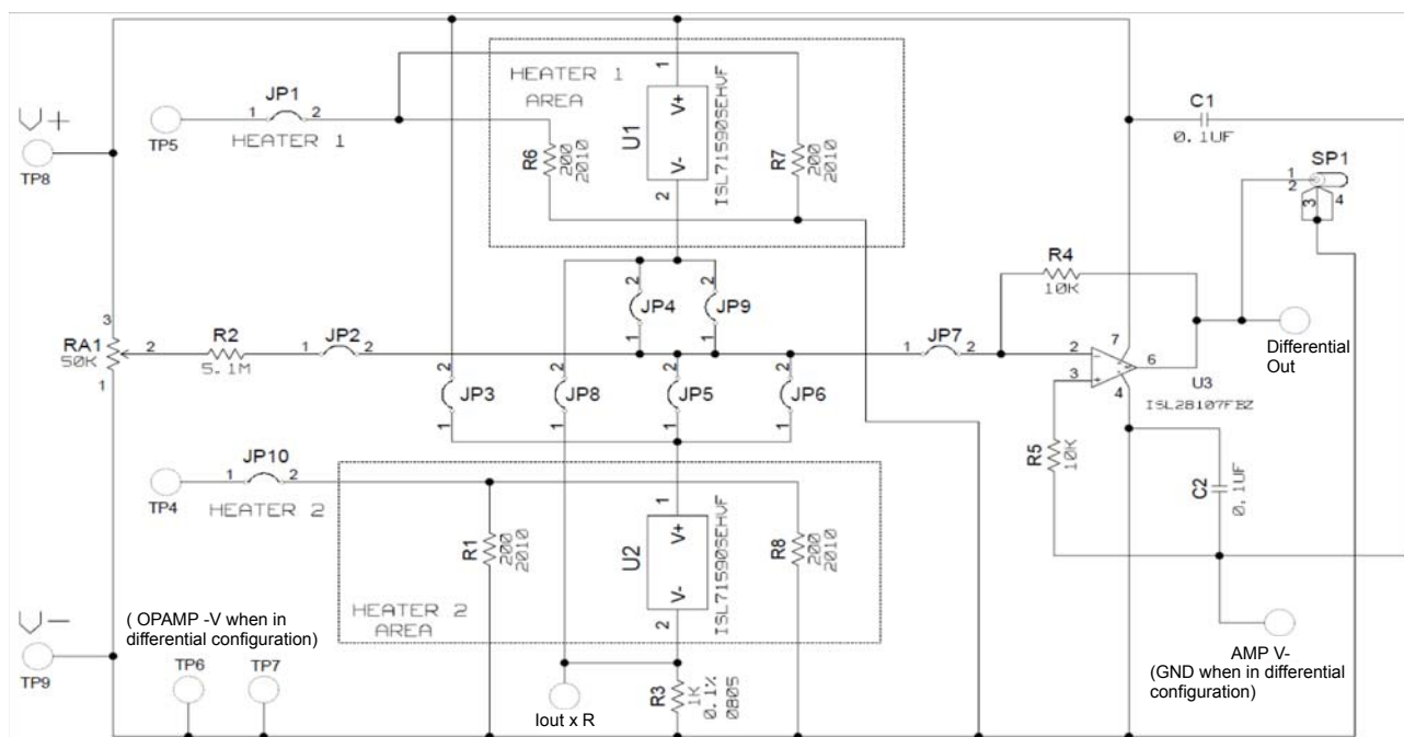
FIGURE 12. ISL71590SEHEV1Z SCHEMATIC
