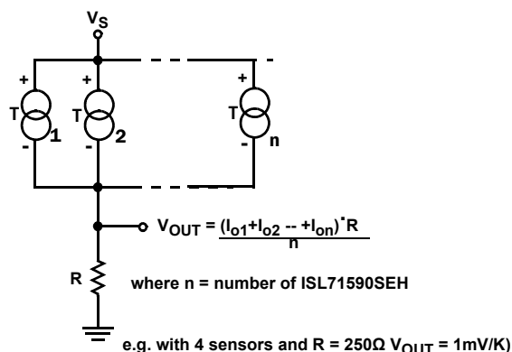
FIGURE 7. AVERAGE TEMPERATURE SENSING SCHEME
