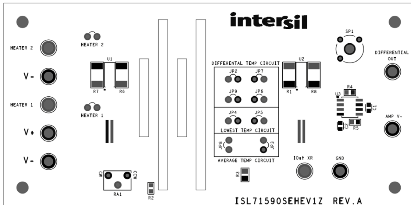
FIGURE 13. ISL71590SEHEV1Z TOP LEVEL PCB PATTERN
