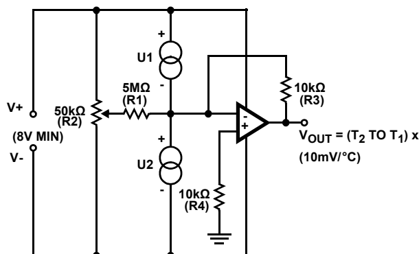
FIGURE 9. DIFFERENTIAL THERMOMETER
