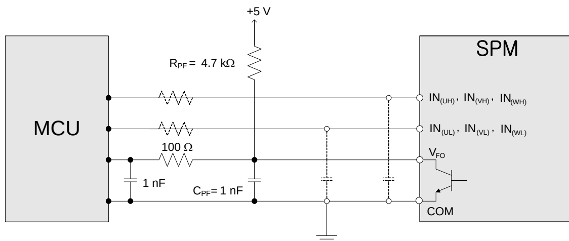
Figure 9. Recommended MCU I/O Interface Circuit
