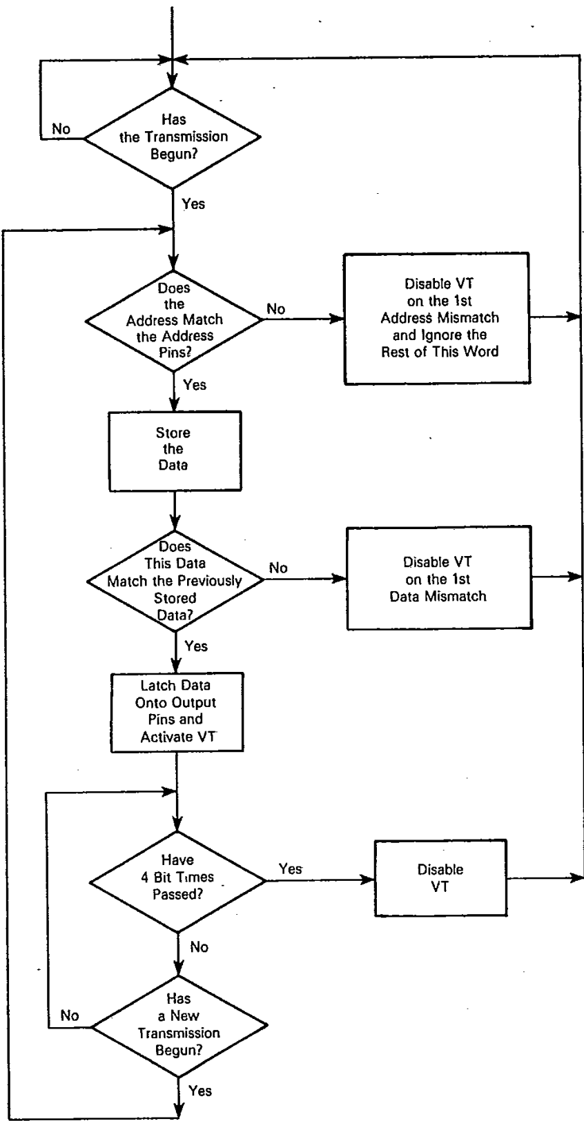
FIGURE 8 — MC145027/MC145029 FLOWCHART
