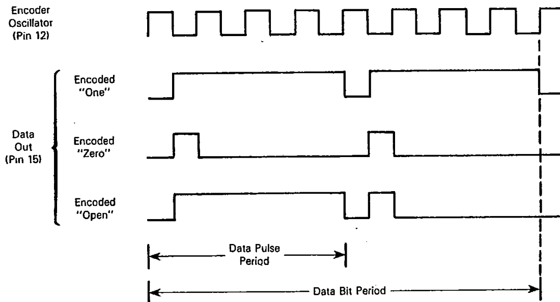
FIGURE 7 — MC145026 ENCODER DATA WAVEFORMS
