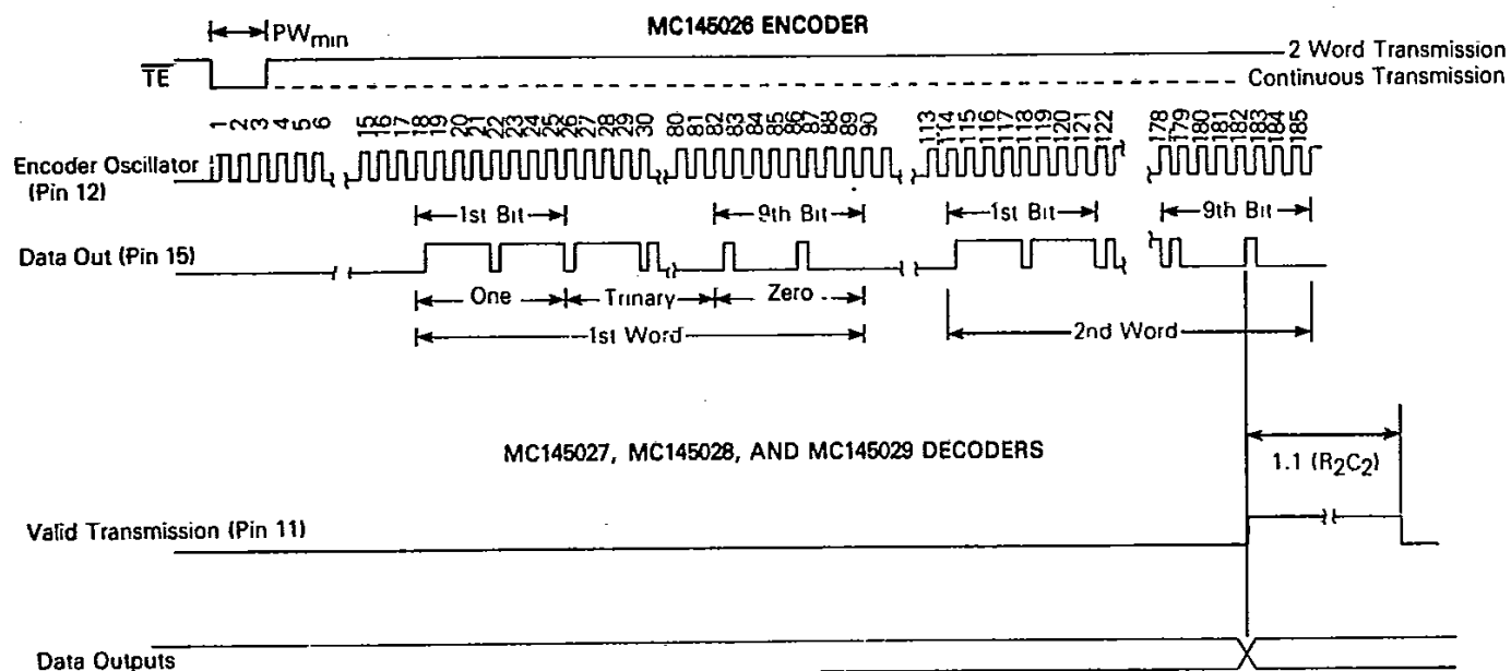
FIGURE 6 — ENCODER/DECODER TIMING DIAGRAM
