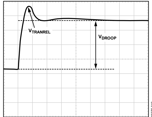
Figure 31. Transient Setting Waveform, Load Release
