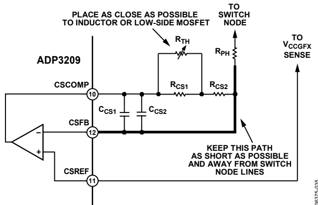
Figure 26. Temperature-Compensation Circuit Values
