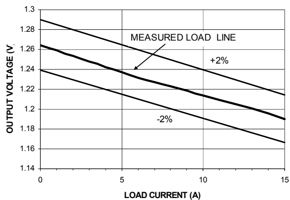
Figure 7. Load Line Accuracy
