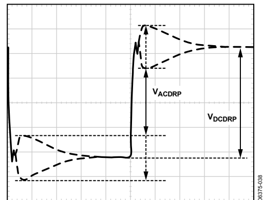
Figure 29. AC Load Line Waveform
