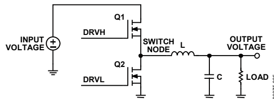
Figure 18. Buck Topology
