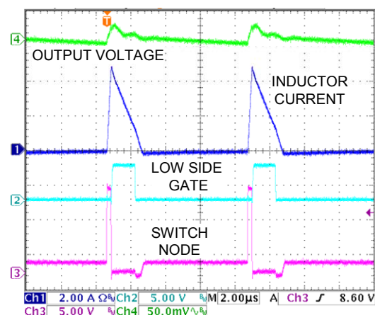
Figure 8. DCM Waveforms, 0.5 A Load Current
