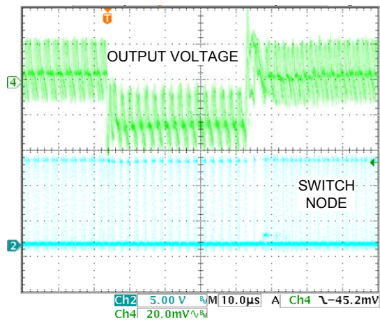
Figure 10. Load Transient, 3 A to 10 A, V_{IN} = 12V
