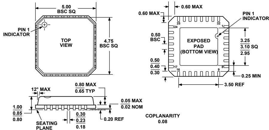
Figure 32. 32-Lead Lead Frame Chip Scale Package [LFCSP_VQ] 5 mm x 5 mm Body, Very Thin Quad (CP-32-2) Dimensions shown in millimeters
