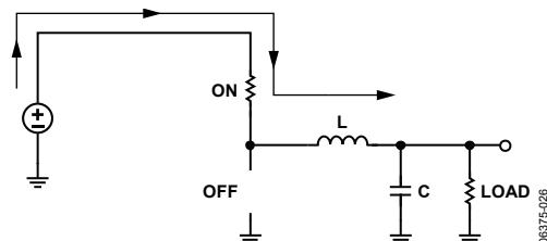
Figure 19. Buck Topology Inductor Current During t_0 and t_1
