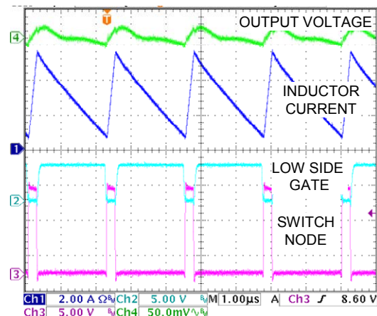
Figure 9. CCM Waveforms, 3 A Load Current
