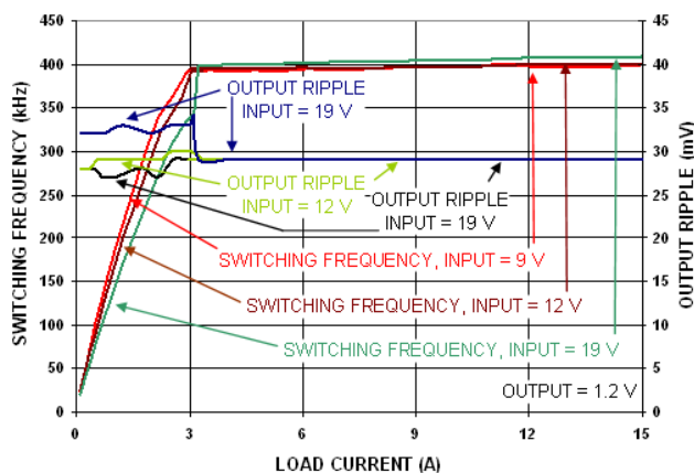
Figure 6. Switching Frequency vs. Input Voltage in RPM Mode
