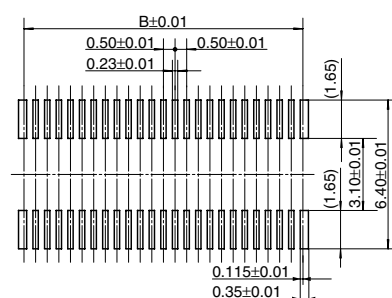
Recommended metal mask pattern Metal mask thickness: Here, 120 μm (Opening area ratio: 76%)
