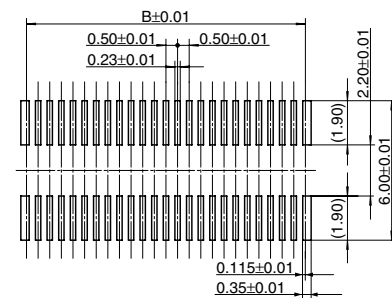
Recommended metal mask pattern Metal mask thickness: Here, 120 μm (Opening area ratio: 87%)
