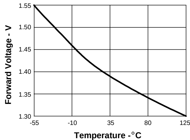
SME2470 Forward Voltage vs Temperature
