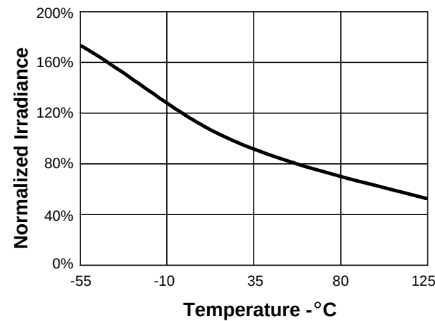
SME2470 Irradiance vs Temperature
