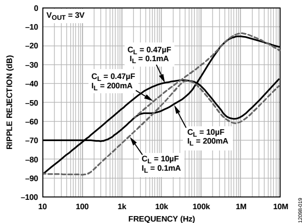
Figure 19. Power Supply Ripple Rejection vs. Frequency
