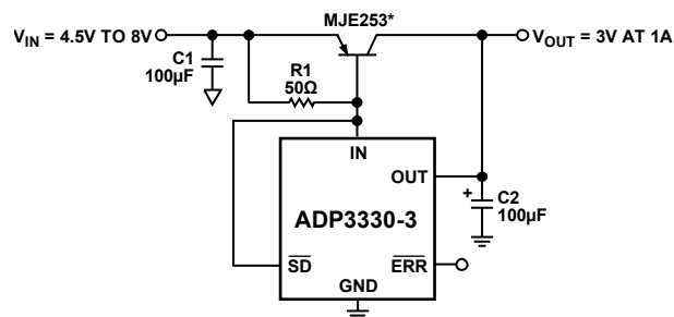
Figure 28. High Output Current Linear Regulator
