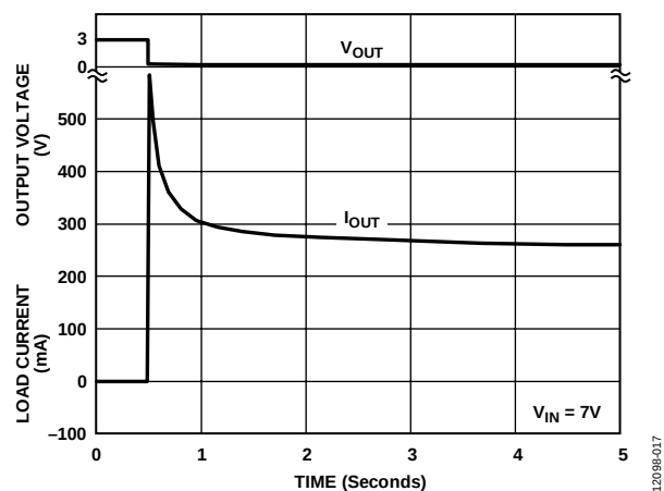
Figure 17. Short-Circuit Current
