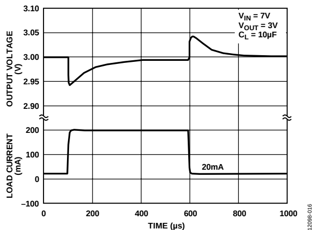
Figure 16. Load Transient Response, C_L = 10\mu F
