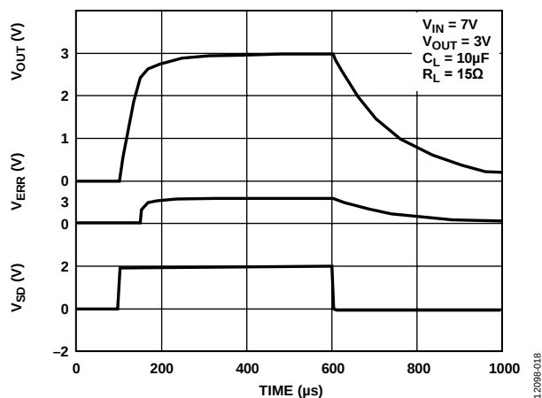
Figure 18. Turn On/Turn Off Response
