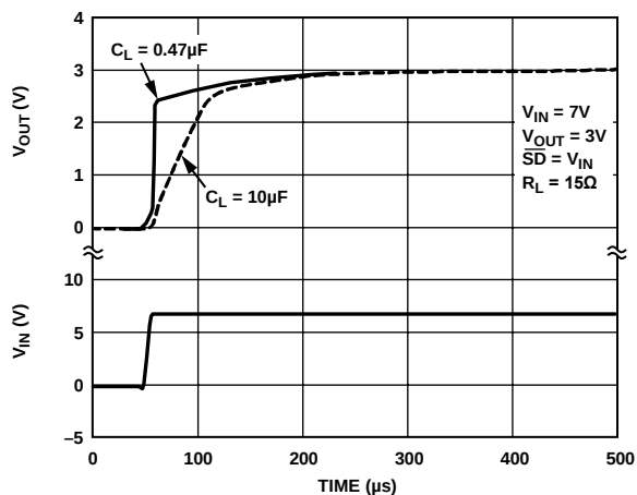
Figure 12. Power-Up Response
