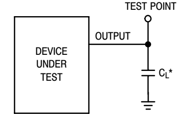
Figure 7. Test Circuit
