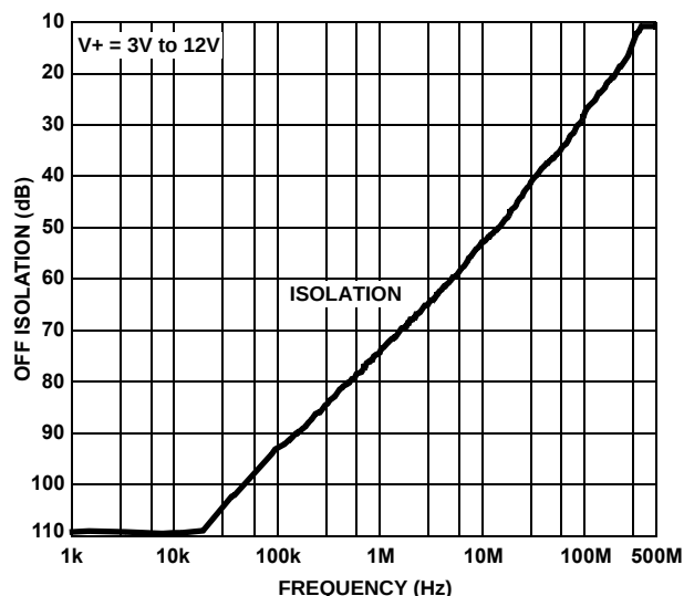
FIGURE 17. OFF ISOLATION
