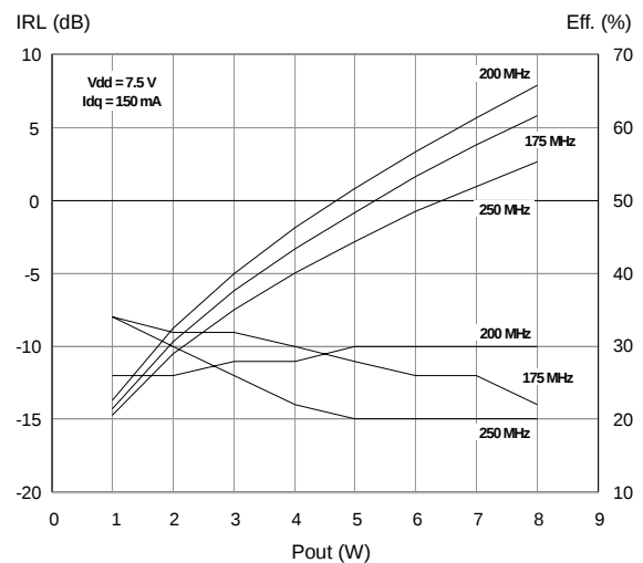
Return Loss and Efficiency vs. Output Power
