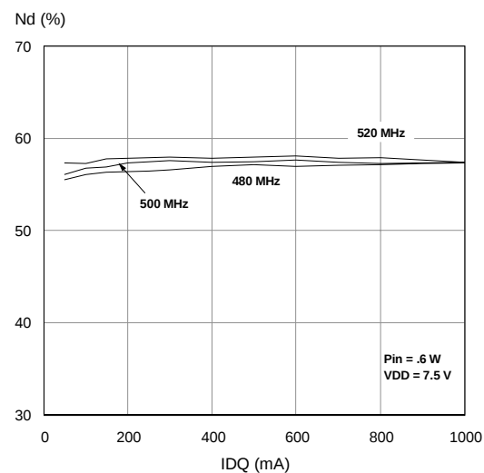
Drain Efficiency vs. Bias Current
