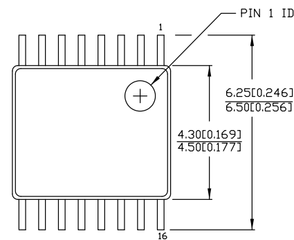
Figure 7. 16-Pin TSSOP 4.40 mm Body Z16.173
