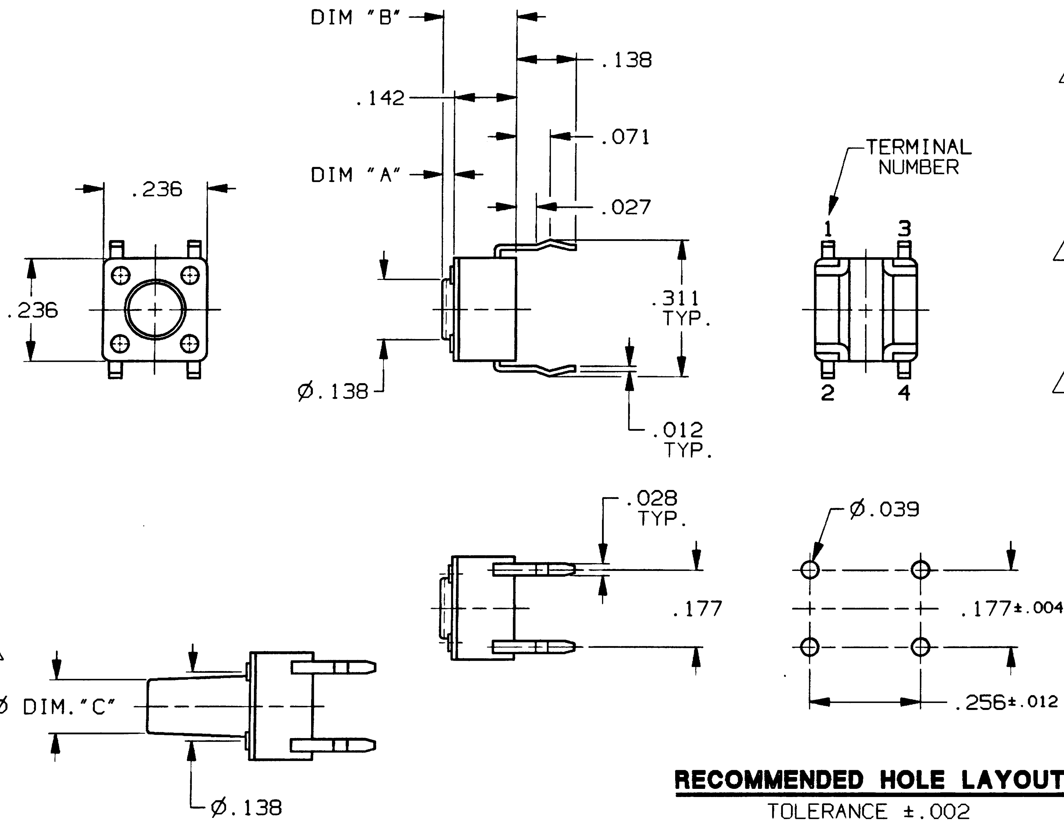
VIEW A-A FSM6J THRU FSM18J
