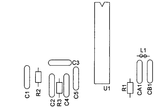
Figure 41. Z86129 Application Circuit with I 2 C
