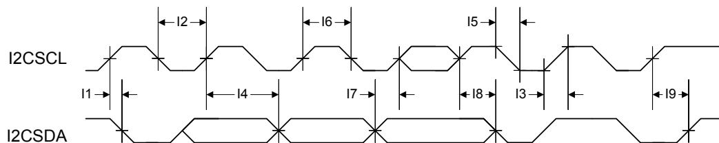
Figure 21-24. I 2 C Timing
