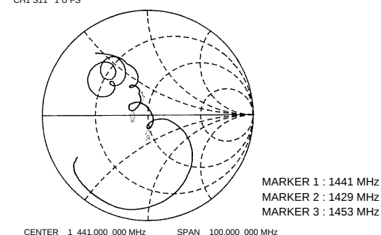
Input Reflection Coefficient vs. Frequency
