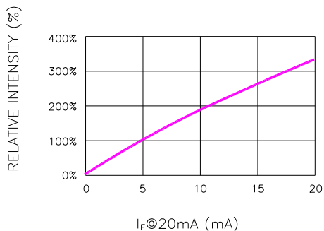
Fig.1 RELATIVE INTENSITY VS. FORWARD CURRENT
