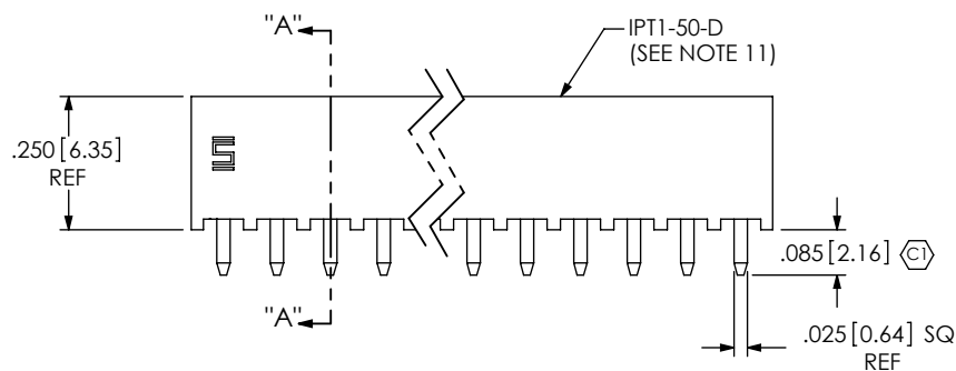
FIG.1 (IPT1-150-01-XX-D-XXX SHOWN)
