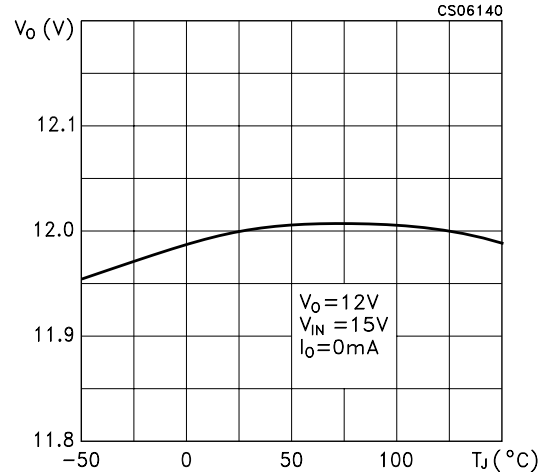
Figure 5 : Load Regulation vs Temperature
