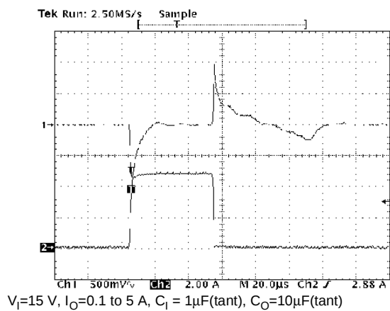
Figure 27 : Load Transient
