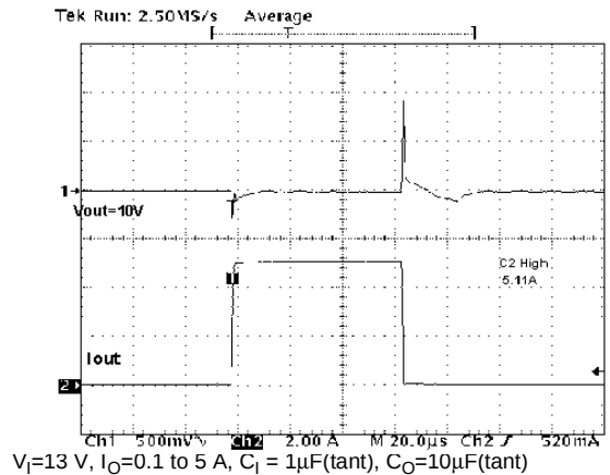
Figure 29 : Load Transient
