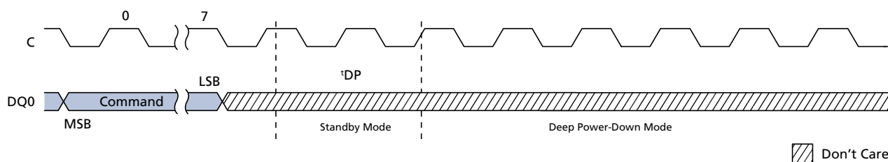
Figure 27: DEEP POWER-DOWN Command Sequence
