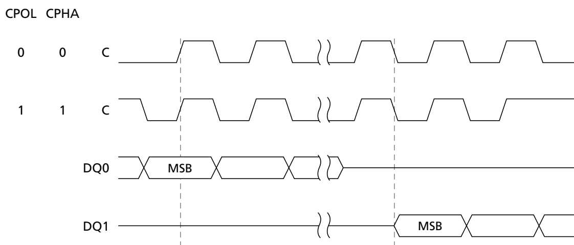
Figure 5: SPI Modes
