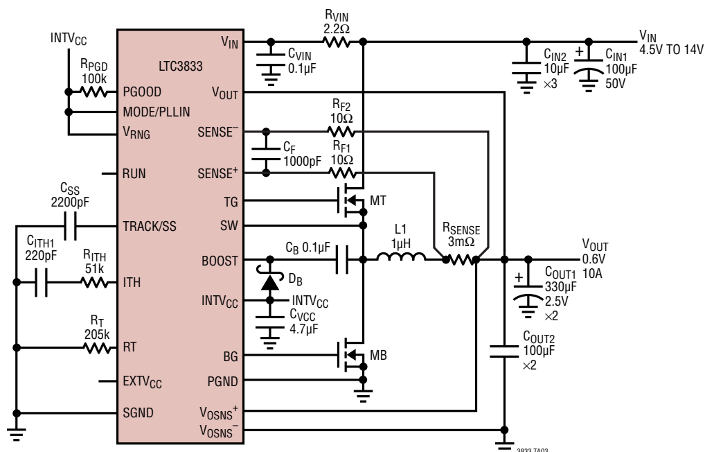
0.6V, 10A, 200kHz Low Output Step-Down Converter
