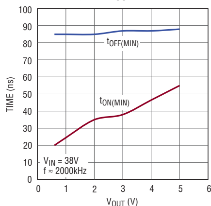
t_{ON(MIN)} and t_{OFF(MIN)} vs Voltage on V_{OUT} Pin
