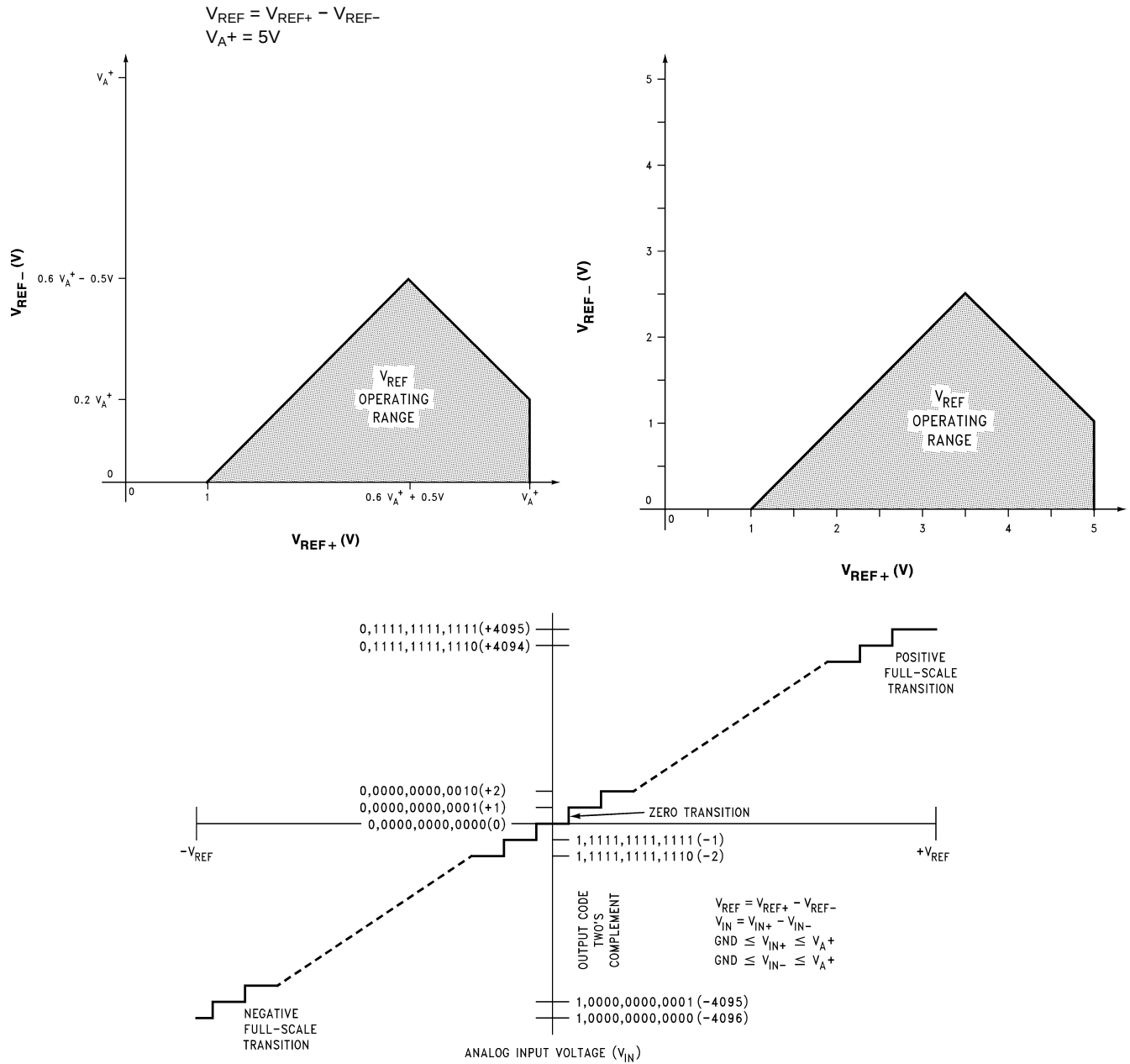
Figure 4. Transfer Characteristic
