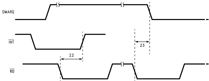
Figure 44. Interrupt and DMARQ
