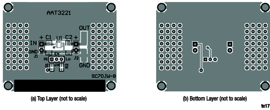
Figure 30: AAT3221 (SC70JW-8) Evaluation Board
