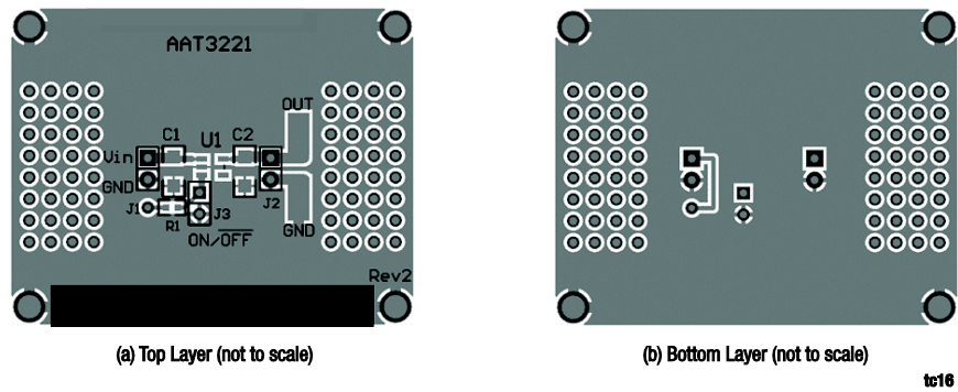
Figure 29: AAT3221 (SOT23-5) Evaluation Board
