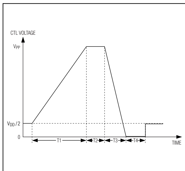
Figure 7. EEPROM Programming
