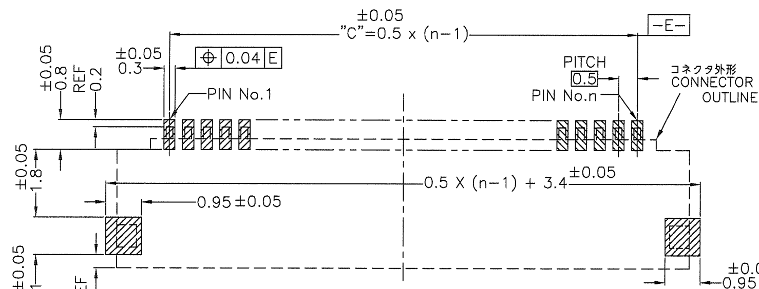
RECOMMENDED PCB PATTERN LAYOUT
