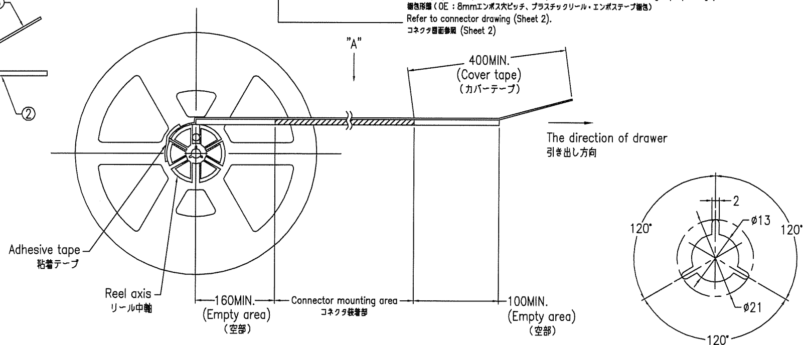
DETAIL "B" (1/1) "B" 部詳細図 (1/1)
