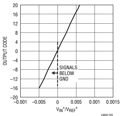
Figure 3. Output Code vs V_{IN}^+ with V_{IN}^- = 0 (LTC2462)
