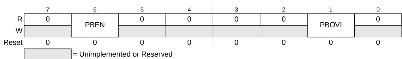
Figure 26-51. 16-Bit Pulse Accumulator B Control Register (PBCTL)
