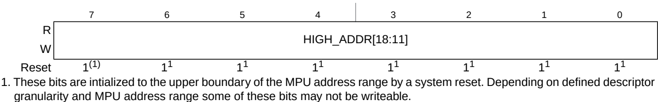
Figure 17-12. MPU Descriptor Register 4 (MPUDESC4)
