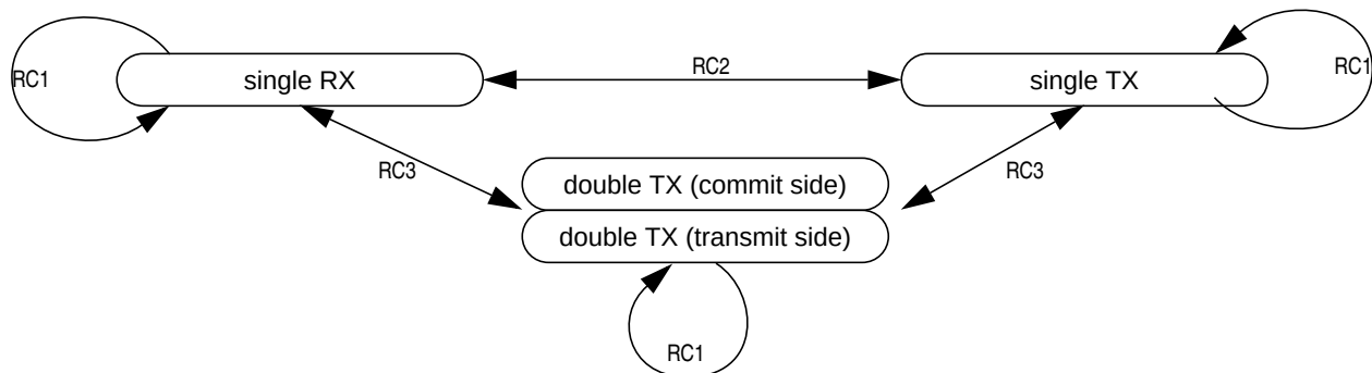
Figure 13-131. Message Buffer Reconfiguration Scheme
