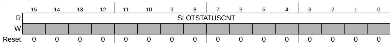
Figure 13-48. Slot Status Counter Registers (SSCR0–SSCR3)
