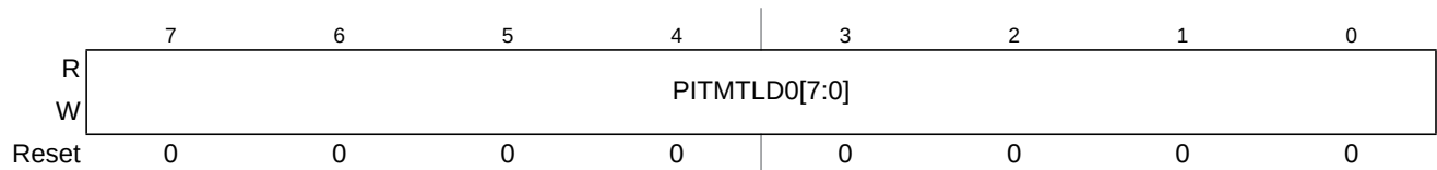
Figure 22-9. PIT Micro Timer Load Register 0 (PITMTLD0)
