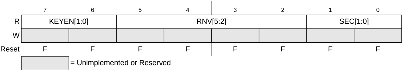
Figure 8-6. Flash Security Register (FSEC)
