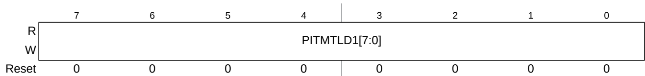
Figure 22-10. PIT Micro Timer Load Register 1 (PITMTLD1)
