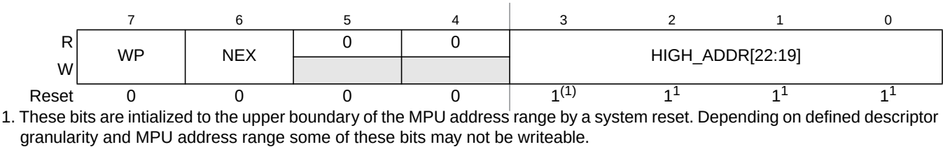
Figure 17-11. MPU Descriptor Register 3 (MPUDESC3)
