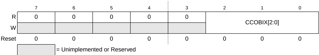
Figure 10-7. FCCOB Index Register (FCCOBIX)
