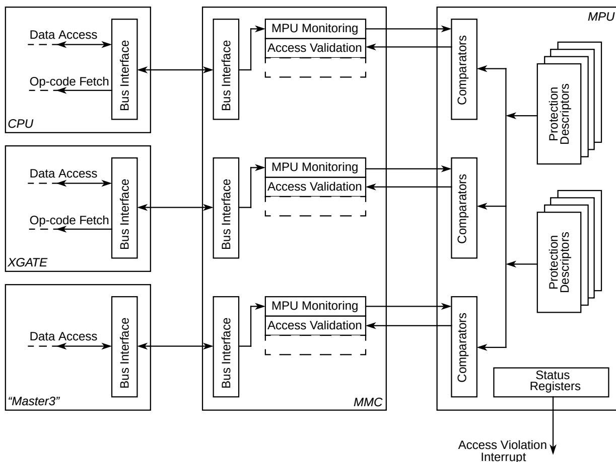
Figure 17-1. Block Diagram
