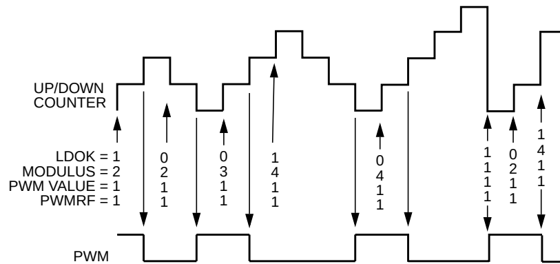
Figure 20-71. Half-Cycle Center-Aligned Modulus Loading
