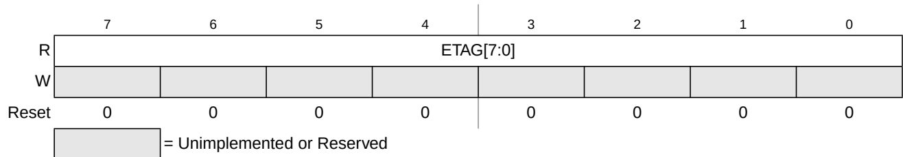
Figure 9-19. EEE Tag Counter Low Register (ETAGLO)
