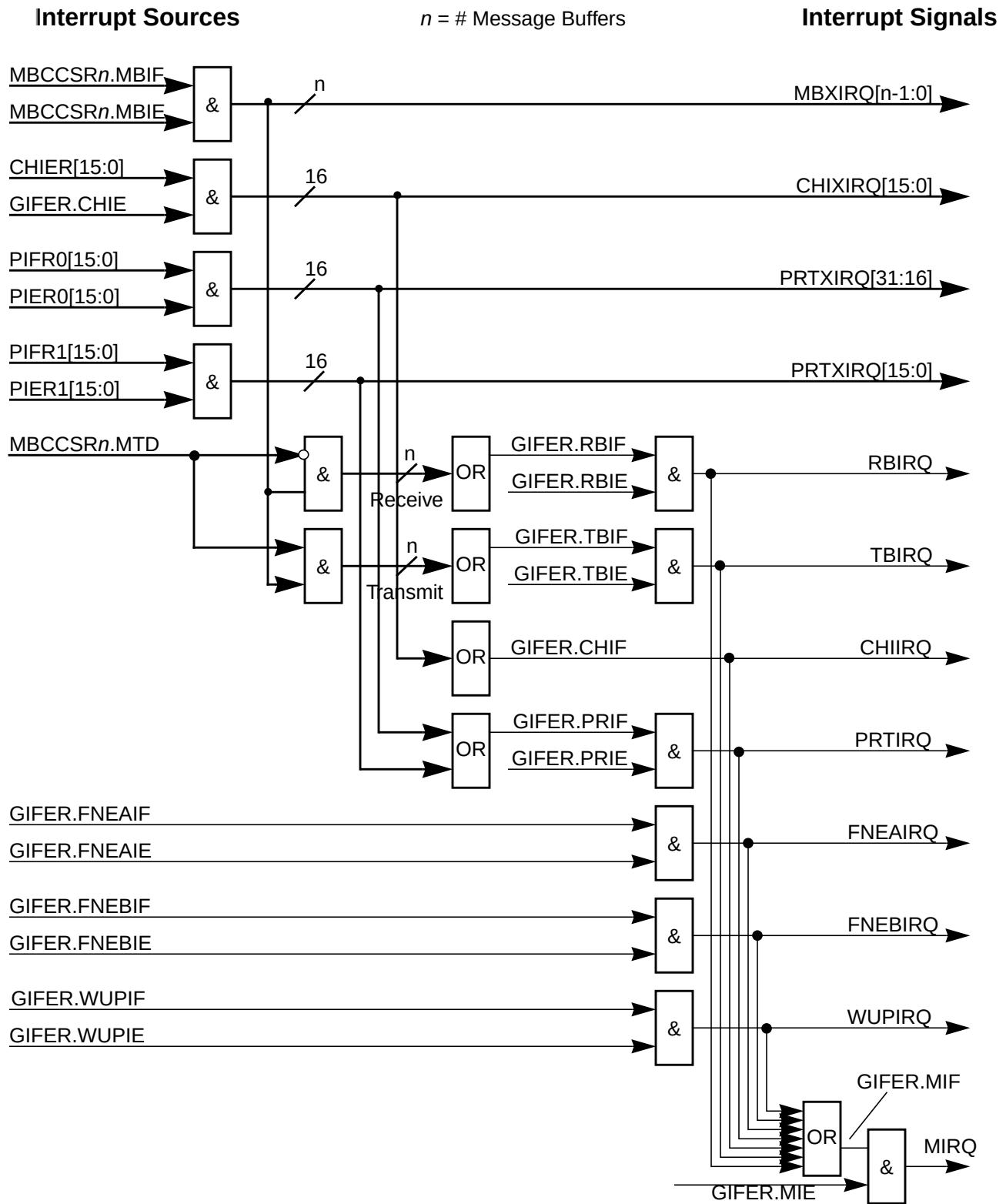
Figure 13-144. Scheme of cascaded interrupt request
