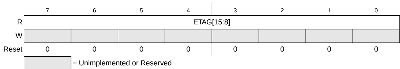
Figure 9-18. EEE Tag Counter High Register (ETAGHI)
