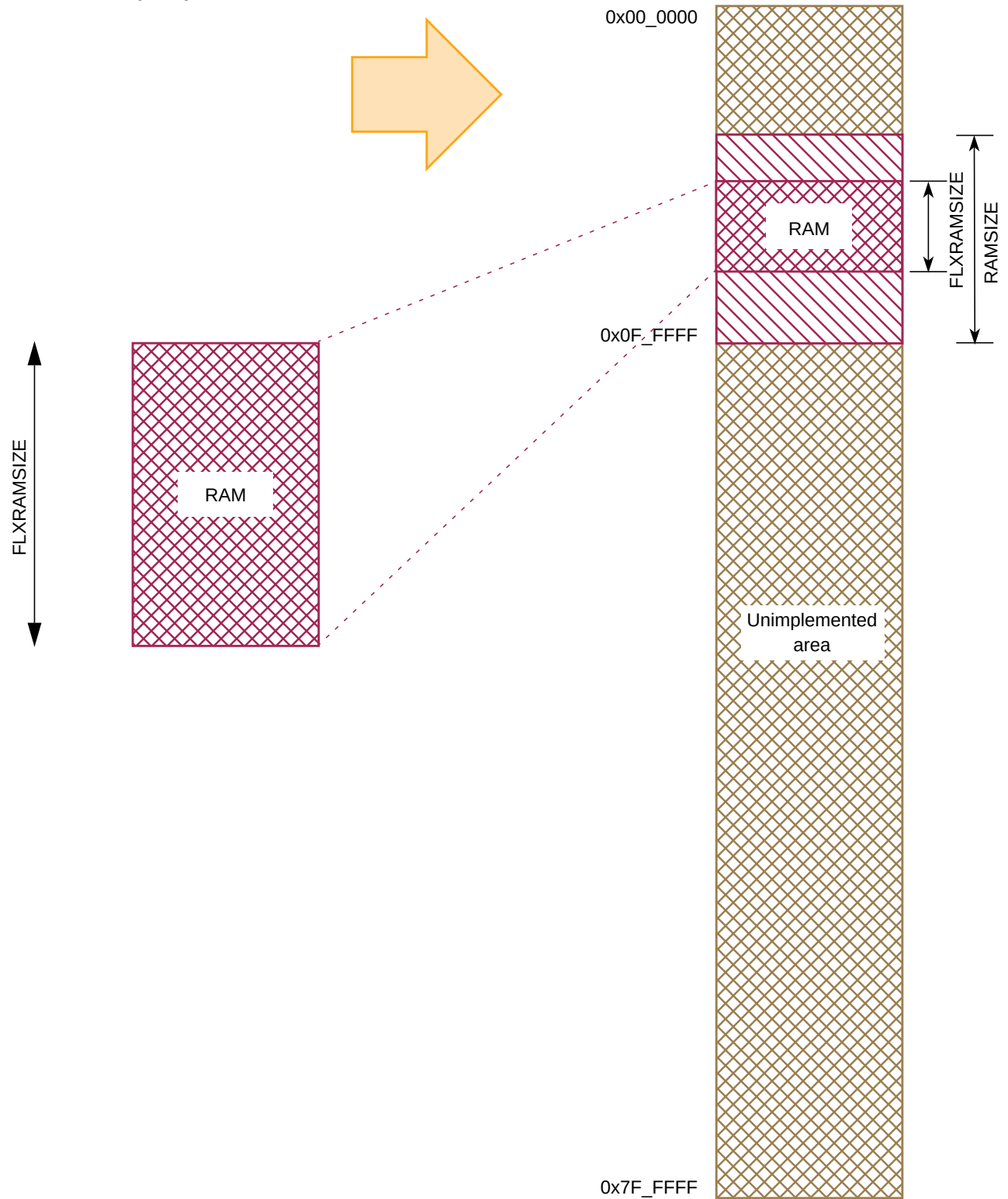
Figure 11-20. FLEXRAY Global Address Mapping
