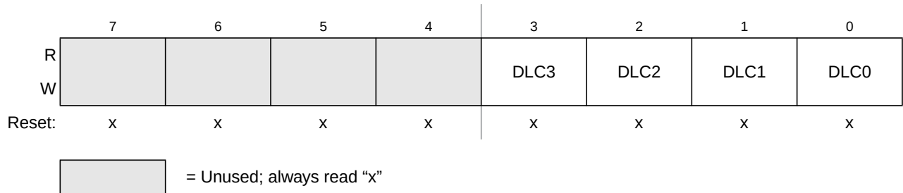
Figure 21-34. Data Length Register (DLR) — Extended Identifier Mapping
