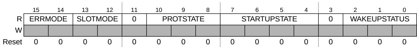
Figure 13-20. Protocol Status Register 0 (PSR0)
