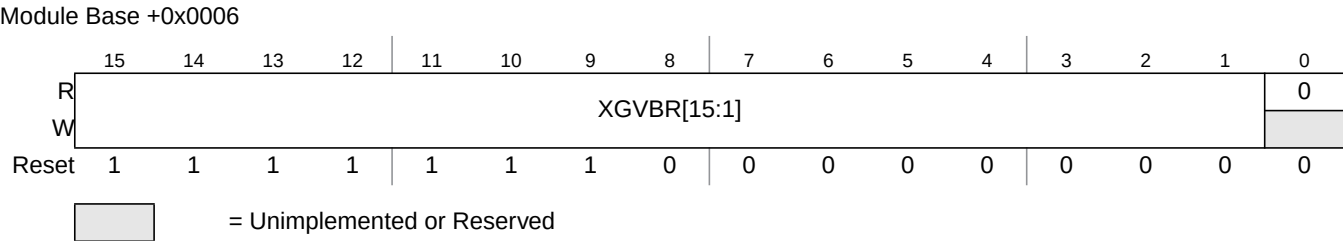
Figure 14-9. XGATE Vector Base Address Register (XGVBR)
